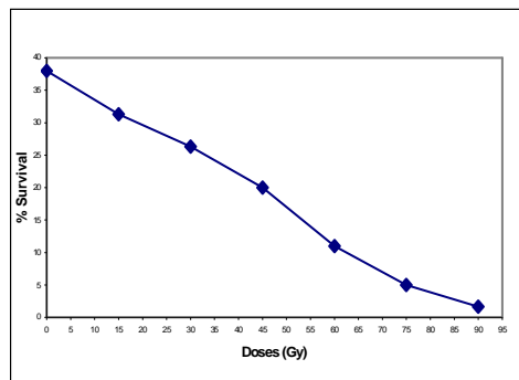
Fig.1: Effect of different doses of Gamma rays on survival percentage of the shoot in guava cv. Safeda
