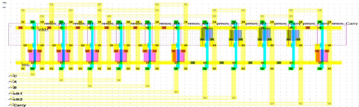
Fig.10: Proposed – Hybrid Full Adder Topology – Carry Function
