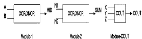
Fig.3: Hybrid Full Adder Modules
