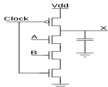
Fig.4: Dynamic Logic Implementation
