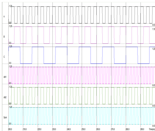
Fig.11: Simulation of Proposed Circuit - Sum Function
