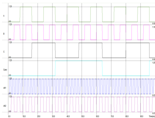
Fig.12: Simulation of Proposed Circuit - Carry Function
