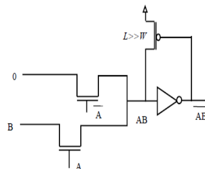
Fig.2: Design of PTL
