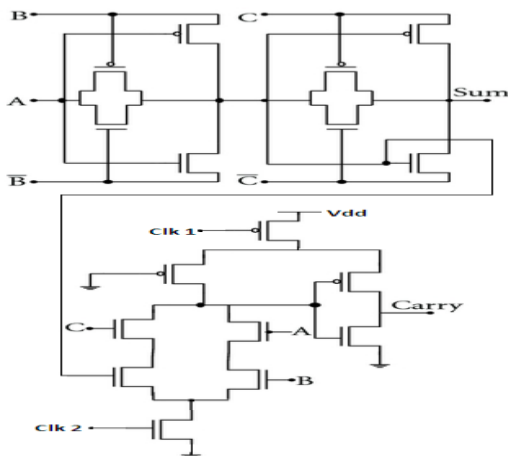
Fig.7: Proposed – Hybrid Full Adder Topology
