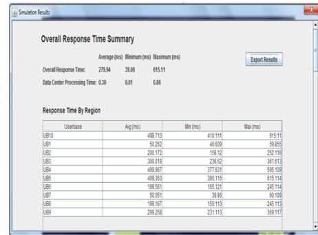
Fig. 9. Overall Response Time Summary (For Fig 8.1)
