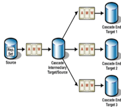
Fig. 1 Data Replication
