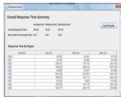
Fig. 11. Overall Response Time Summary (For Fig 8.3)
