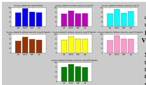
Figure 3: Comparison of Accuracy for different Classifiers by using attributes obtained by Existing and Proposed Algorithm
